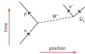
A neutron decays into a proton by the emission of an electron and an electron antineutrino (shown with the arrow moving downwards because it is an antiparticle). The decay is mediated by the negative W boson.
