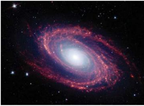
▲ Figure 5 The spiral galaxy M81.
