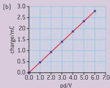
▲ Figure 3(a) and (b) Charging a capacitor with constant current.
