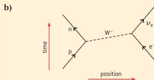
▲ Figure 17 Feynman diagram for an proton–electron collision.
