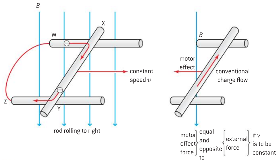
▲ Figure 4 Conductor rod rolling in a magnetic field.
