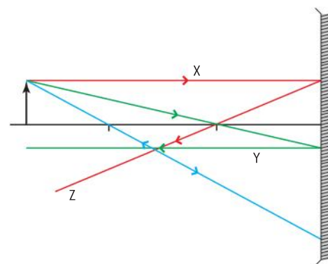
▲ Figure 4 Predictable rays.
