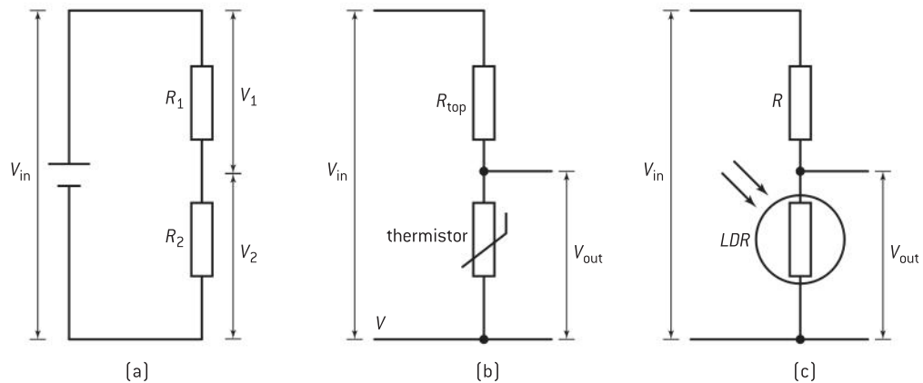
▲ Figure 13 The potential divider.
