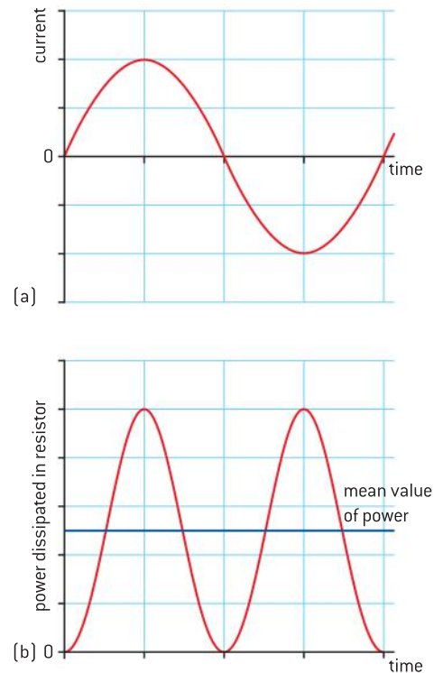
▲ Figure 5 Current–time and power–time graphs for ac.
