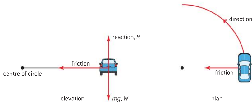
▲ Figure 11 Car moving in a circle.
