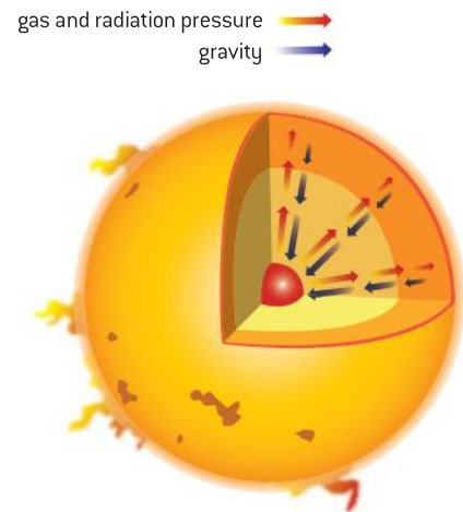
▲ Figure 4 Hydrostatic equilibrium.
