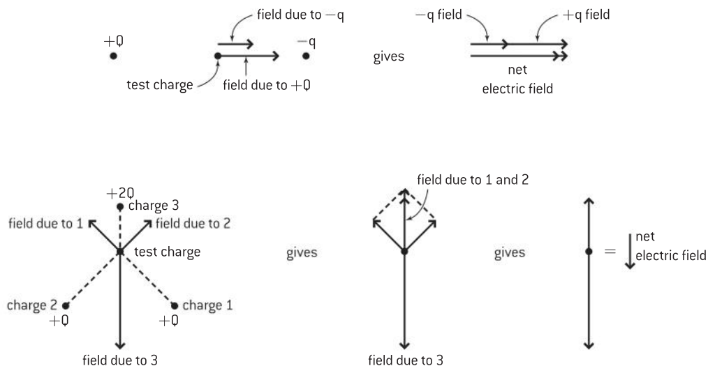
▲ Figure 11 Vector addition of electric fields.
