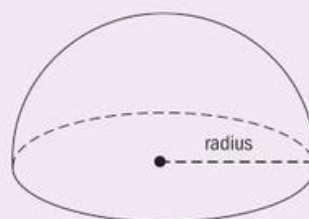
Hemisphere
