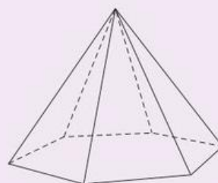
Hexagonal-based pyramid
