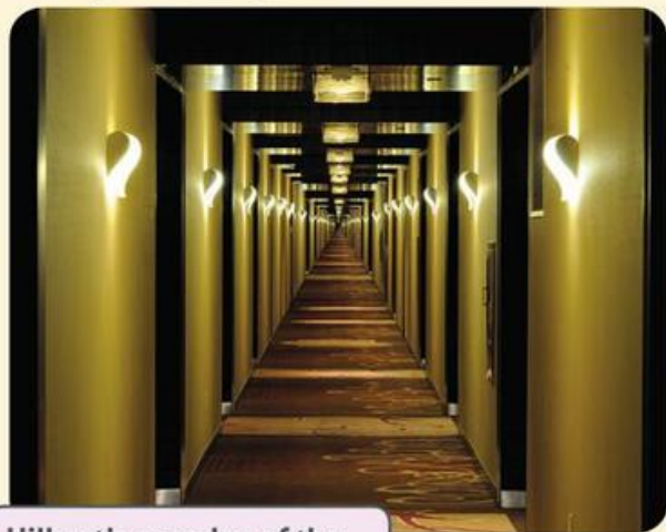
Hilbert's paradox of the grand hotel
